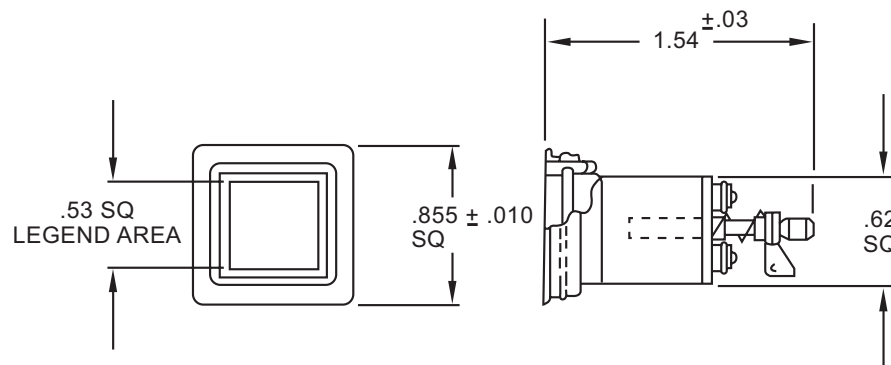
Pushbutton with seal detail.
