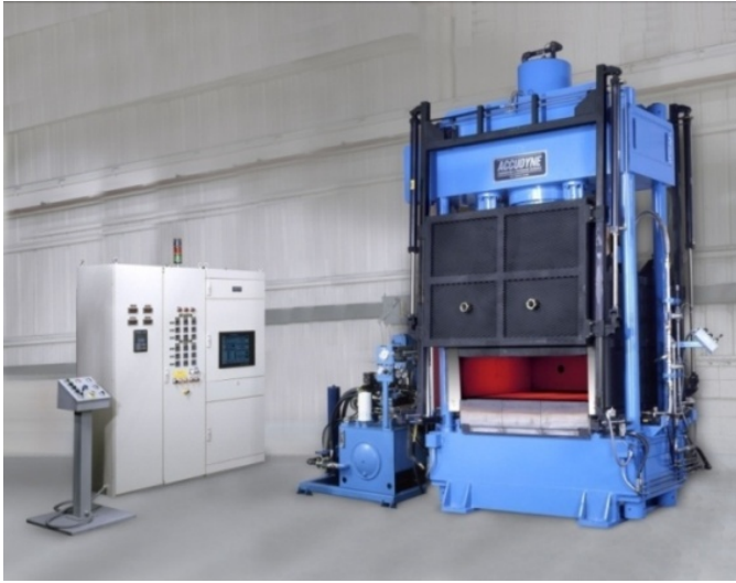
Wisconsin Die Pre-Heat Oven
